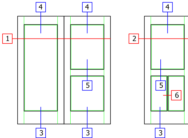
WS-500 STILE DETAIL-SINGLE DOOR
