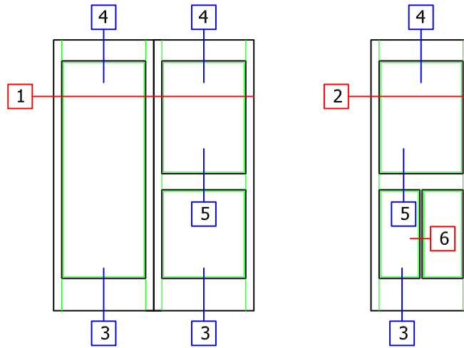
NS-250 STILE DETAIL-PAIR DOORS
